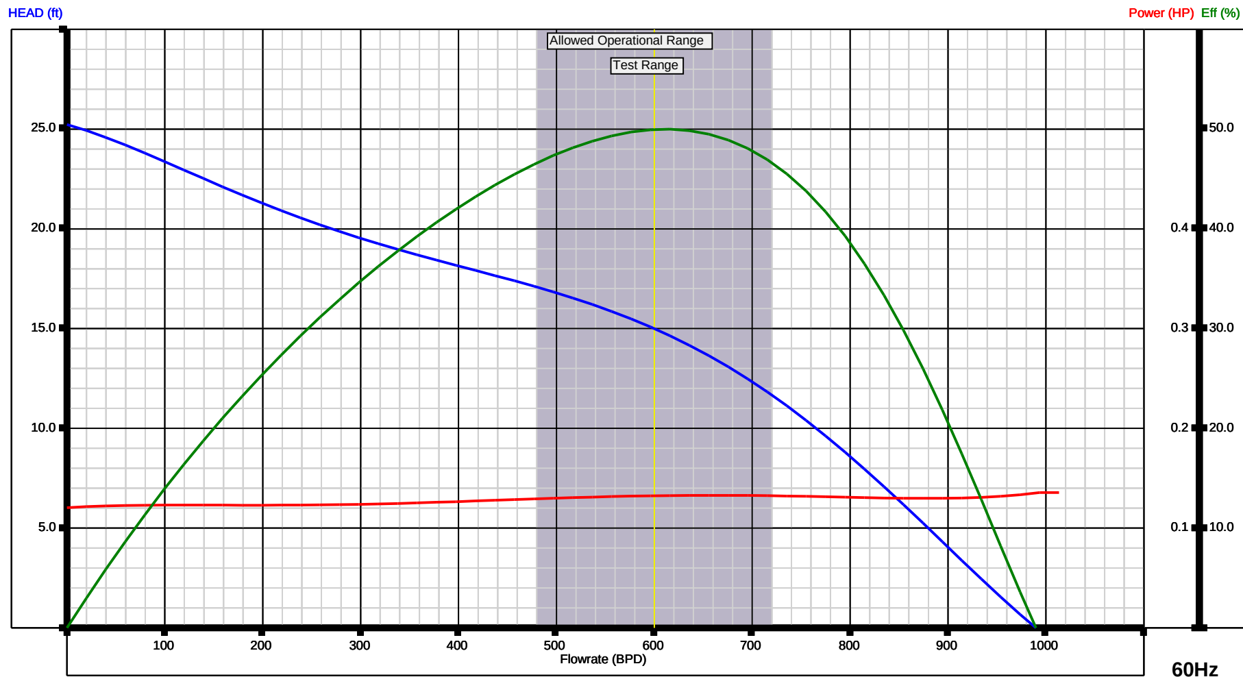
FLEX6 Pump 338 SERIES 1 Stage Performance Curve RPM=3500 Sp.Gr.=1.0
